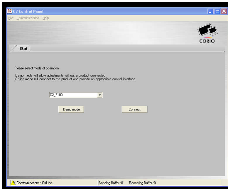
Figure 3 Main screen
