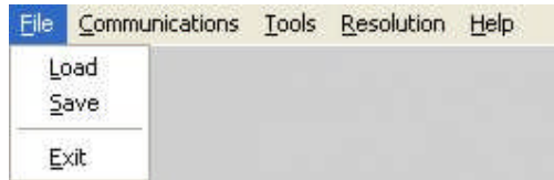
Figure 6 File menu
