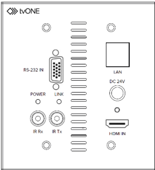
1T-CT-653-USWP Transmitter
