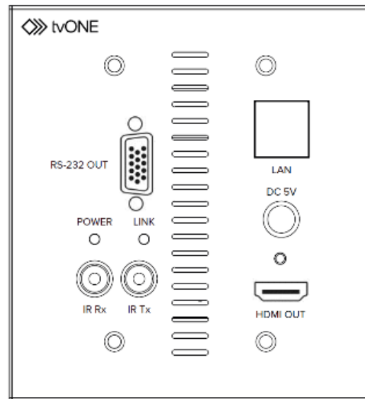
1T-CT-654-USWP Receiver
