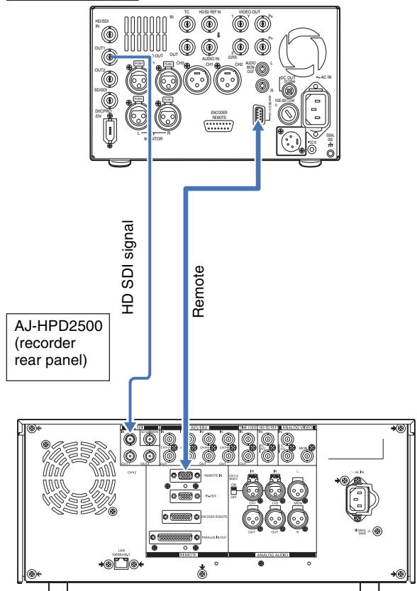
AJ-HD1400, etc. (source rear panel)
