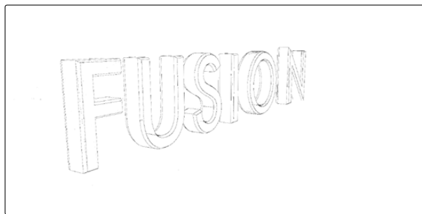
Z-Coverage channel
