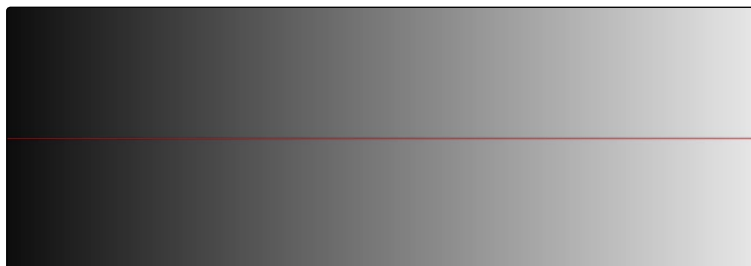
Linear Gradient
