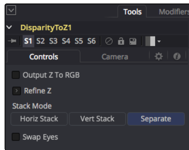
DisparityToZ Controls
