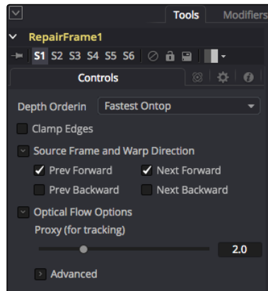
RepairFrame Controls
