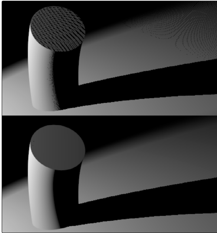
Top: Results of shadow map Z-fighting Bottom: Corrected shadow shown using Biasing
