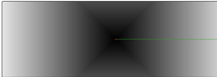
Square Gradient
