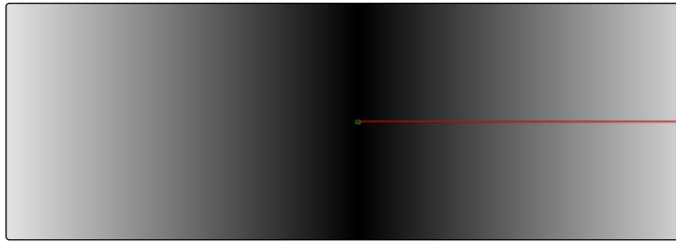
Reflect Gradient
