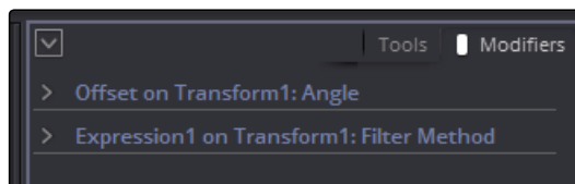
Modifier panel
