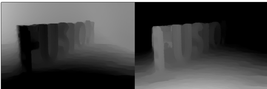
XY Disparity
