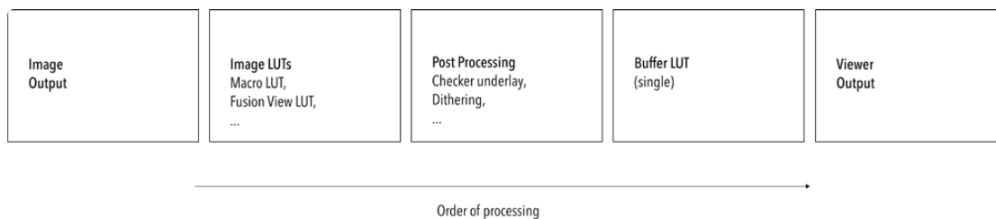
The order of processing for 2D images and 3D scenes.
