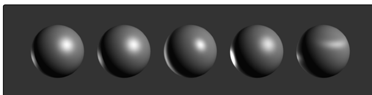
Illumination models L to R: Standard, Blinn, Phong, Cook-Torrance and Ward
